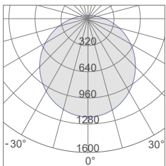
TPL-4T32JF Photometric
