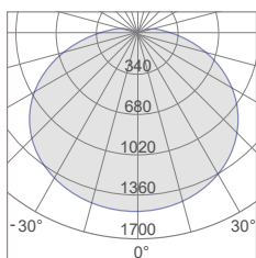
TPL-4M36 Photometric
