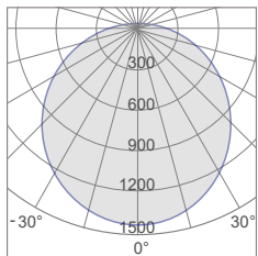
TPL-4J36S Photometric
