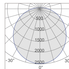
TPL-4L48B Photometric
