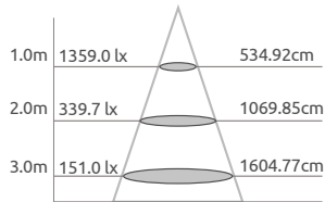
TPL-2R18-XTJ-φ70
