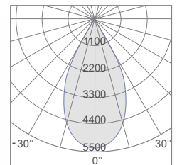
TPL-4L50B-P 60° Photometric
