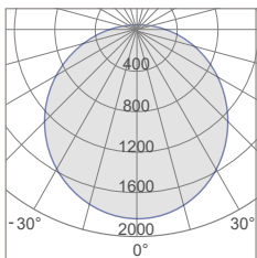
TPL-5L45A Photometric
