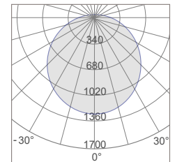
TPL-2D18M Photometric
