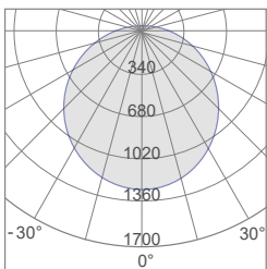
TPL-4J18SA-E Photometric
