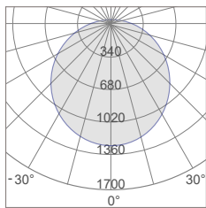
TPL-4J18A-E Photometric
