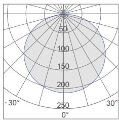
CLB18-B Photometric
