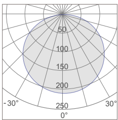
CLD-25 Photometric
