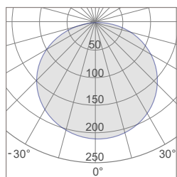
CLC-24 Photometric
