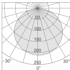
CLA-18 Photometric
