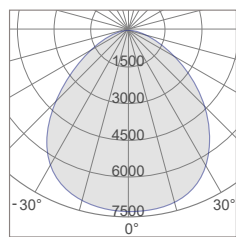
HBA150 Photometric
