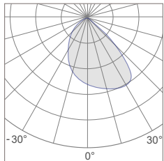
SLA120 Photometric
