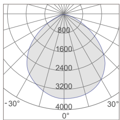
FLA100 Photometric
